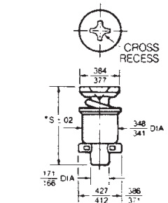
Typical 40 series stud, Part No. 6080-xx S=.62+(.03 x Dash No.)
