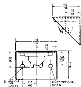
Side Mount 40 series receptacle, Part No. 6087
