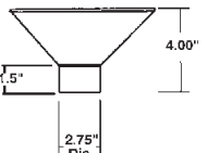
Headlight Mount Air Inlet Part No. 3623
