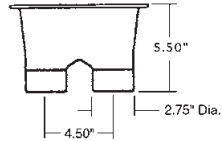
Small Bumper Mounted Inlet Part No. 3625
