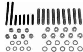
Left: Rear Stud Kit, Part No. 1413-2
