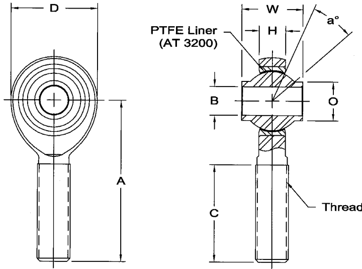
Aurora HXAM (Right Hand) / HXAB (Left Hand) High-Misalignment Rod Ends, Male Threaded Shanks
